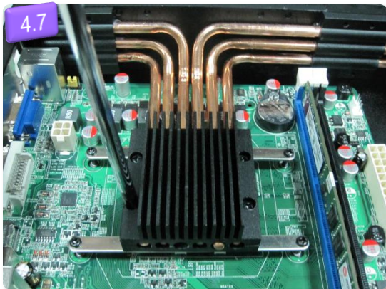
4.7 Coving motherboard cooling panels (up) (A) , Locking 4 screws (M)
