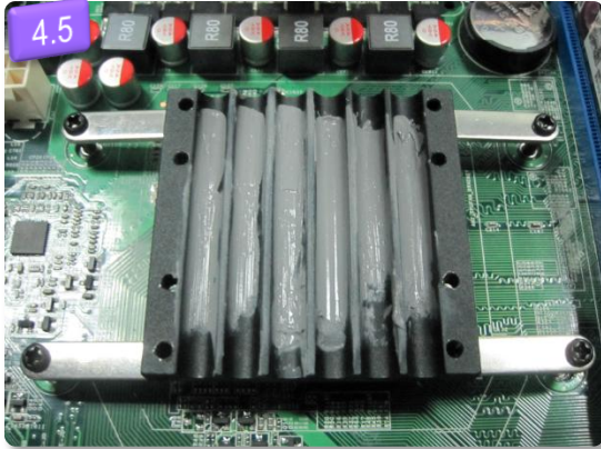
4.5 Wearing thermal grease on cooling panels' V bay.
