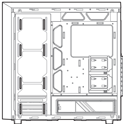
Side : Supports 120/140mm fanx3 or 120/140/240/280/360/420 Radiator(280 radiator installed)
